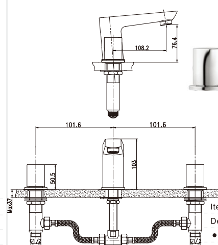
Item Nr. NA1143L0 Description: Basin tap • Brass body. Chrome plating. • G1/2" ceramic valve. For cold water.
