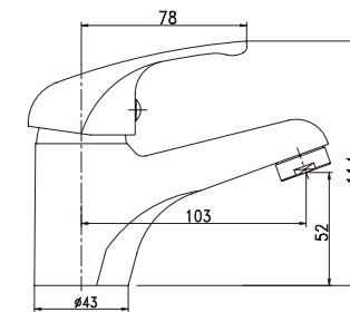
Item Nr. BJ001300 Description Basin mixer • Brass body. Chrome plating. • \Phi 35mm ceramic cartridge.
