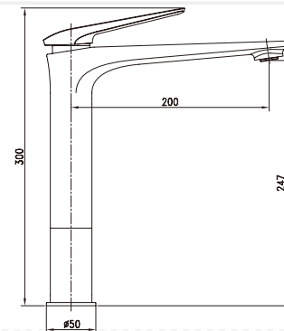
Item Nr.: PF1833A2 Chrome or Black finish Description: Basin mixer.High model • Brass body. Chrome plating or Black finish. • Ø35mm ceramic cartridge.
