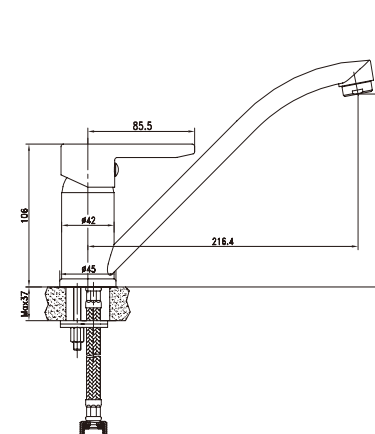
Item Nr. FU077520 Description Kitchen sink mixer: • Brass body, Chrome plating.Brass swivel spout. • 35mm ceramic cartridge.
