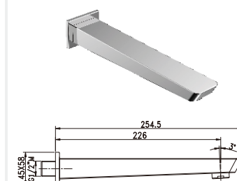
Item Nr. PD2043RT3 Description Spout. • Brass. Chrome plating. • G1/2" M wall connection
