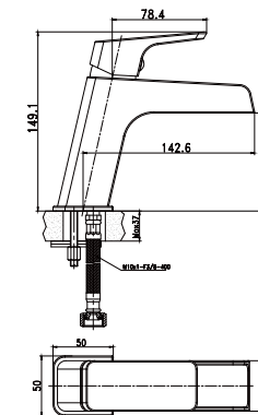
Item Nr. PD204320 Description Basin mixer. Waterfall water outlet. • Brass body. Chrome plating. • 35mm ceramic cartridge.
