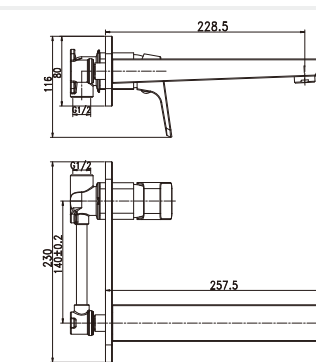
Item Nr. PD2043R3 Description Wall basin mixer. • Brass body. Chrome plating. Brass spout. • \Phi 35mm ceramic cartridge.
