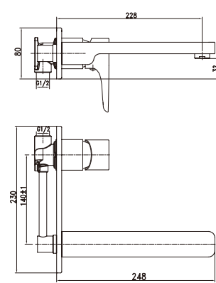
Item Nr. DP0723R0 Description Wall basin mixer. • Brass body. Chrome plating. Brass spout. • \Phi 40mm ceramic cartridge.
