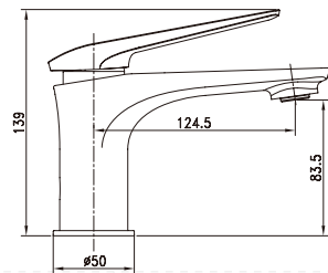
Item Nr.: PF183300 Chrome or Black finish Description: Basin mixer • Brass body. Chrome plating or Black finish. • Ø35mm ceramic cartridge.
