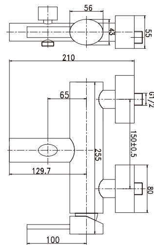
Item Nr. CE045100 Description Bath mixer • Brass body.Chrome plating. • Ø35mm ceramic cartridge.
