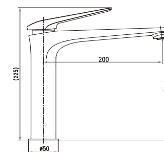
Item Nr.: PF1833A0 Bronze or Copper finish Description: Basin mixer.High model • Brass body. Bronze or Copper finish. • Ø35mm ceramic cartridge.
