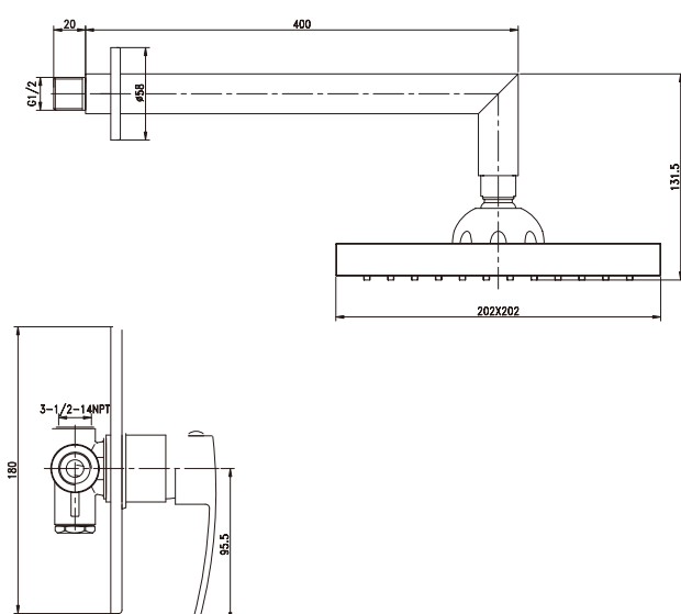
Item Nr. AE0787R0 Description Wall Shower mixer • Brass body, Chrome plating. • Ø35mm ceramic cartridge. • Brass shower arm.
