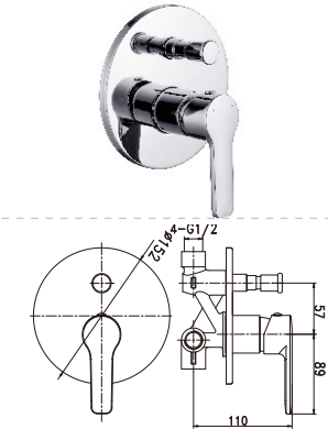
Item Nr. KC1111RB Description Built - in bath mixer. • Brass body. Chrome plating. Ø 35mm cartridge .
