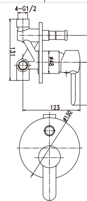
Item Nr. CV500900 Description Built-in bath & shower mixer • Brass body. Chrome plating. • \Phi 40mm ceramic cartridge.
