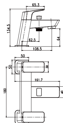
Item Nr. PD2041Y0 Description Two handle Bath & Shower mixer • Brass body. Chrome plating. • G3/4" ceramic valve.
