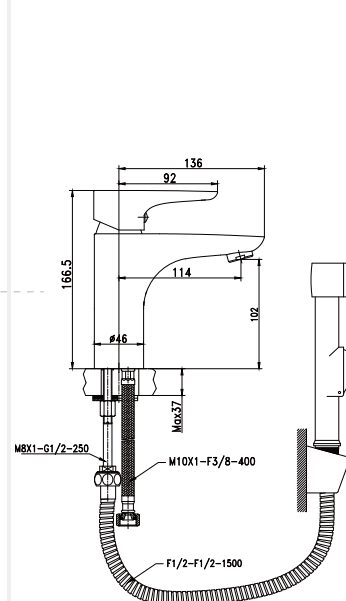
Item Nr. DP072330 Description Basin mixer with shattaf • Brass body. Chrome plating. • \Phi 40mm ceramic cartridge.
