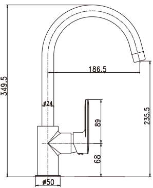
Item Nr. KC111500 Description Kitchen sink mixer • Brass body. Chrome plating. Brass swivel spout. • Ø35mm ceramic cartridge.
