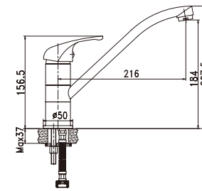
Item Nr. BJ0015A0 Description Kitchen sink mixer. • Brass body. Chrome plating. Brass swivel spout. • \Phi 35mm ceramic cartridge.
