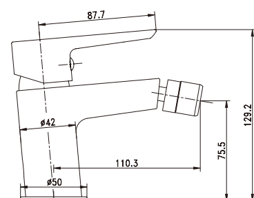
Item Nr. NA114400 Description: Bidet mixer • Brass body. Chrome plating. • \Phi 35mm ceramic cartridge.
