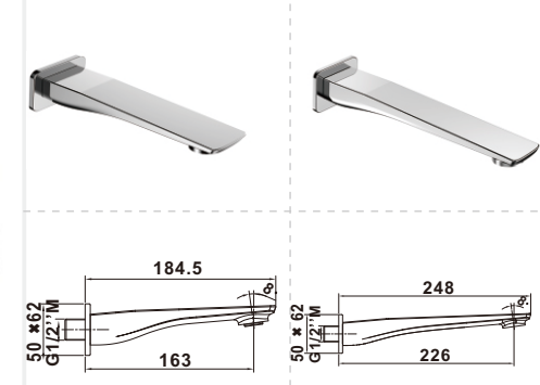
Item Nr. PF1833RT Description: Spout • Brass body.Chrome plating. • G1/2"M wall connection.
