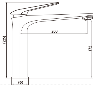
Item Nr.: PF1833A0 Chrome or Black finish Description: Basin mixer.High model • Brass body. Chrome plating or Black finish. • Ø35mm ceramic cartridge.
