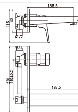
Item Nr. PD2043R0 Description Wall basin mixer. • Brass body. Chrome plating. Brass spout. • \Phi 35mm ceramic cartridge.
