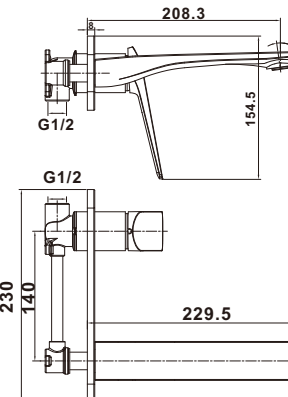
Item Nr. PF1833R0 Description: Wall basin mixer • Brass body.Chrome plating.Brass spout. • Ø35mm ceramic cartridge.
