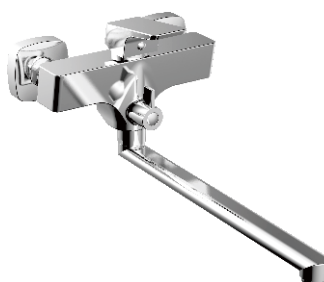
Item Nr. PD2049A0 Description Bath mixer with diverter • Brass body. Brass swivel spout. Chrome plating. • \Phi 35mm ceramic cartridge.
