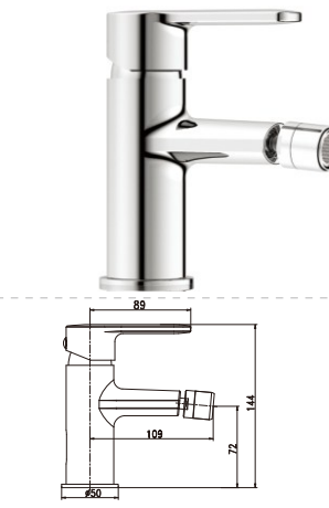
Item Nr. KC111400 Description Bidet mixer • Brass body. Chrome plating. 35mm cartridge.
