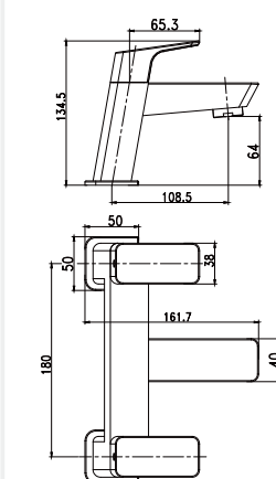
Item Nr. PD2041Y0 Description Two handle Bath & Shower mixer • Brass body. Chrome plating. • G3/4" ceramic valve.
