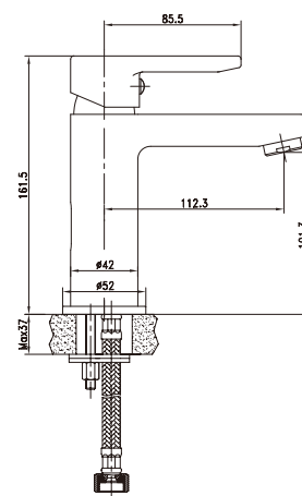
Item Nr. FU077320 Description Basin mixer: • Brass body, Chrome plating. • 35mm ceramic cartridge.
