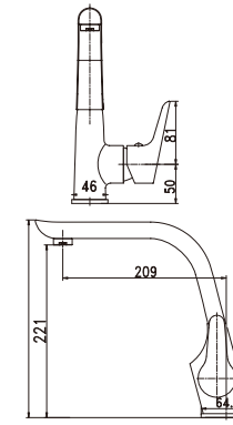
Item Nr. BJ0015A0 Description Kitchen sink mixer. • Brass body. Chrome plating. Brass swivel spout. • \Phi 35mm ceramic cartridge.
