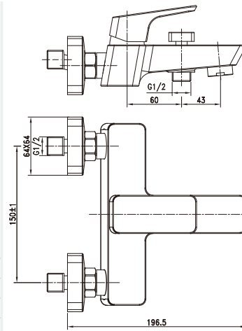
Item Nr. PD204100 Description Bath mixer. • Brass body. Chrome plating. • \Phi 35mm ceramic cartridge.
