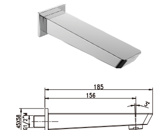
Item Nr. PD2043RT Description Spout. • Brass. Chrome plating. • G1/2" M wall connection
