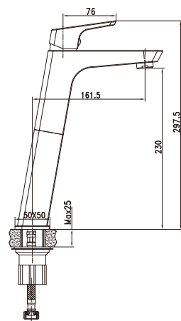
Item Nr. PD2043A0 Description Basin mixer. High model. • Brass body. Chrome plating. • \Phi 35mm ceramic cartridge.
