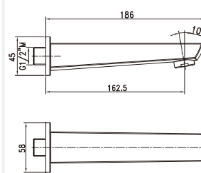
Item Nr. NA1141RT2 Description: Spout. • Brass. Chrome plating. • G1/2" M wall connection.
