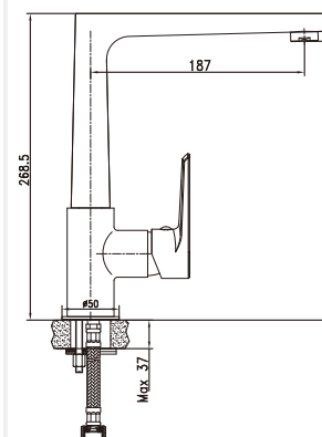
Item Nr. NA114530 Description: Kitchen sink mixer. • Brass body. Chrome plating. Brass swivel spout. • \Phi 35mm ceramic cartridge.
