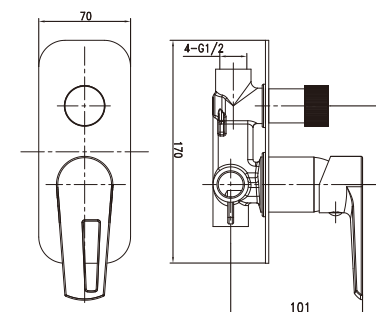
Item Nr. NA1141RB3 Description: Built - in bath mixer. Brass body. Chrome plating. 35mm ceramic cartridge.
