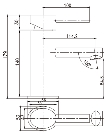
Item Nr. CE045300 Description Basin mixer • Brass body.Chrome plating. • Ø35mm ceramic cartridge.
