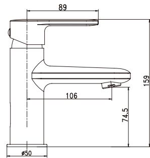
Item Nr. KC111300 Description Basin mixer • Brass body. Chrome plating. • Ø35mm ceramic cartridge.
