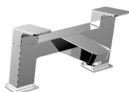
Item Nr. PD2049A0 Description Bath mixer with diverter • Brass body. Brass swivel spout. Chrome plating. • \Phi 35mm ceramic cartridge.
