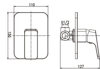
Item Nr. PD2047RB Description Built-in shower mixer. • Brass body. Chrome plating. • \Phi 35mm ceramic cartridge.
