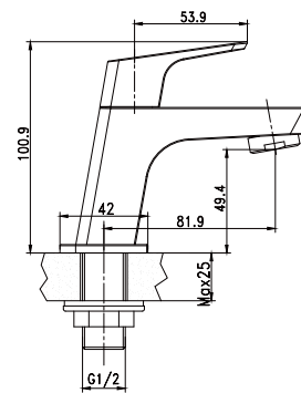
Item Nr. PD204330 Description Basin tap per pairs • Brass body. Chrome plating. • G1/2" ceramic valve.
