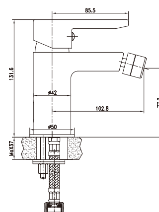
Item Nr. FU077420 Description Bidet mixer: • Brass body, Chrome plating. • 35mm ceramic cartridge.
