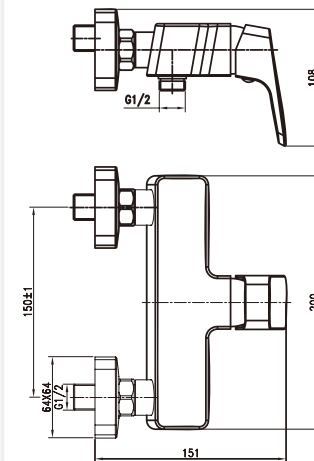
Item Nr. PD204700 Description Shower mixer. • Brass body. Chrome plating. • \Phi 35mm ceramic cartridge.
