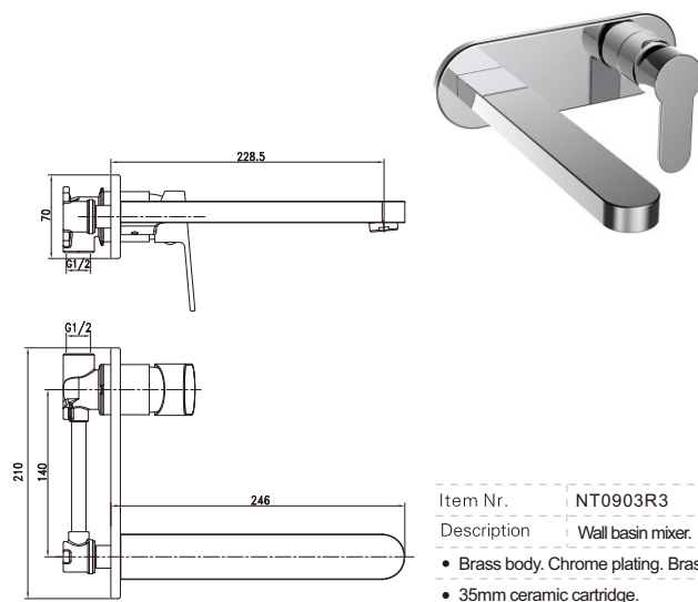
Item Nr. NT0903R0 Description Wall basin mixer. • Brass body. Chrome plating. Brass spout. • \Phi 35mm ceramic cartridge.
