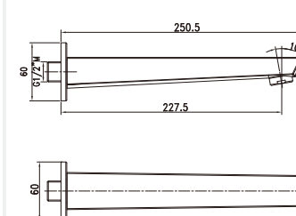
Item Nr. NA1141RT3 Description: Spout. • Brass body. Chrome plating. • G1/2" M wall connection.
