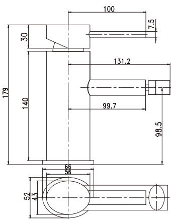
Item Nr. CE045400 Description Bidet mixer • Brass body.Chrome plating. • Ø35mm ceramic cartridge.
