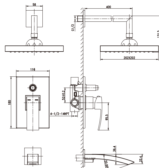
Item Nr. AE0781R0 Description Wall Bath&Shower mixer • Brass body, Chrome plating. • Ø35mm ceramic cartridge. • Brass shower arm. With brass spout.
