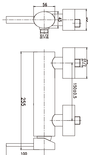
Item Nr. CE045700 Description Shower mixer • Brass body.Chrome plating. • Ø35mm ceramic cartridge.
