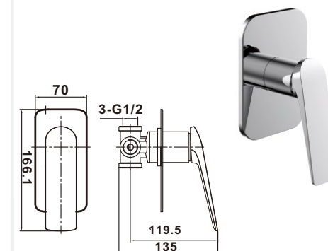
Item Nr. PF1837RB Description: Built-in shower mixer • Brass body.Chrome plating. • Ø35mm ceramic cartridge.
