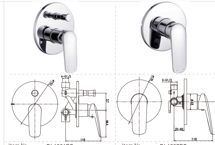
Item Nr. DL1261RB Description Built-in bath mixer. • Brass body. Chrome plating. • \Phi 35mm ceramic cartridge.
