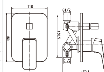
Item Nr. PD2041RB Description Built-in bath mixer. • Brass body. Chrome plating. • \Phi 35mm ceramic cartridge.
