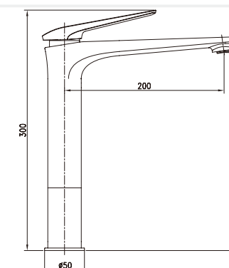
Item Nr.: PF1833A2 Bronze or Copper finish Description: Basin mixer.High model • Brass body. Bronze or Copper finish. • Ø35mm ceramic cartridge.
