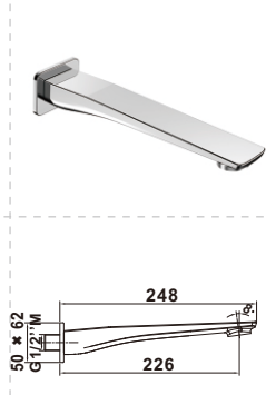
Item Nr. PF1833RT3 Description: Spout • Brass body.Chrome plating. • G1/2"M wall connection.
