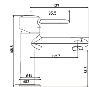
Item Nr. CV063300 Description Basin mixer • Brass body. Chrome plating. • \Phi 40mm ceramic cartridge.
