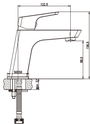
Item Nr. PD204300 Description Basin mixer. • Brass body. Chrome plating. • \Phi 35mm ceramic cartridge.
