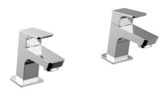
Item Nr. PD204340 Description Basin tap per pairs • Brass body. Chrome plating. • G3/4" ceramic valve.
