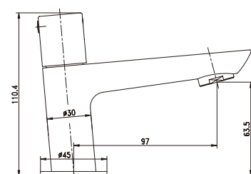
Item Nr. NA1143L0 Description: Basin tap • Brass body. Chrome plating. • G1/2" ceramic valve. For cold water.
