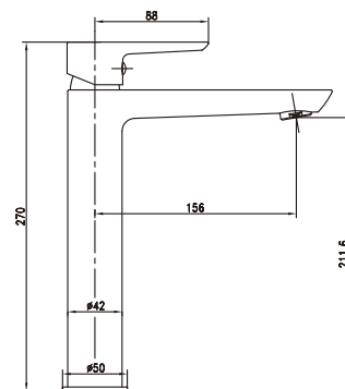
Item Nr. NA1143L3 Description: Basin tap • Brass body. Chrome plating • \Phi 35mm ceramic cartridge. For cold water
