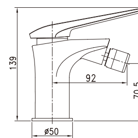
Item Nr. PF183400 Description: Bidet mixer. • Brass body.Chrome plating. • Ø35mm ceramic cartridge.
