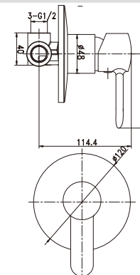
Item Nr. CV500800 Description Built-in Shower mixer • Brass body. Chrome plating. • \Phi 40mm ceramic cartridge.
