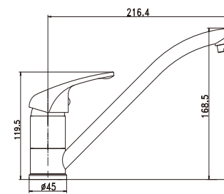
Item Nr. BJ001500 Description Kitchen sink mixer • Brass body. Chrome plating. Brass swivel spout. • \Phi 35mm ceramic cartridge.
