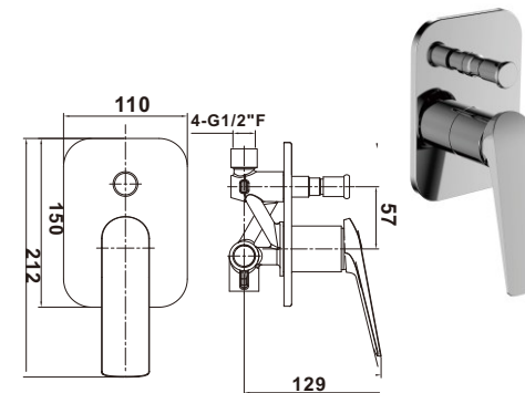
Item Nr. PF1831RB Description: Built-in bath mixer • Brass body.Chrome plating. • Ø35mm ceramic cartridge.
