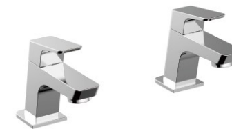
Item Nr. PD204330 Description Basin tap per pairs • Brass body. Chrome plating. • G1/2" ceramic valve.
