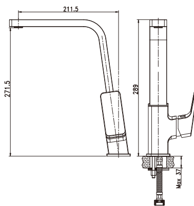
Item Nr. PD204500 Description Kitchen sink mixer. • Brass body. Chrome plating. Brass swivel spout. • \Phi 35mm ceramic cartridge.
