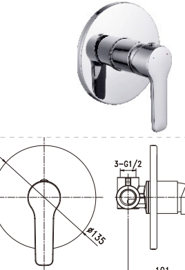
Item Nr. KC1117RB Description Built - in Shower mixer. • Brass body. Chrome plating. Ø 35mm cartridge .
