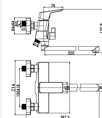
Item Nr. PD204500 Description Kitchen sink mixer. • Brass body. Chrome plating. Brass swivel spout. • \Phi 35mm ceramic cartridge.
