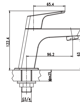
Item Nr. PD204340 Description Basin tap per pairs • Brass body. Chrome plating. • G3/4" ceramic valve.
