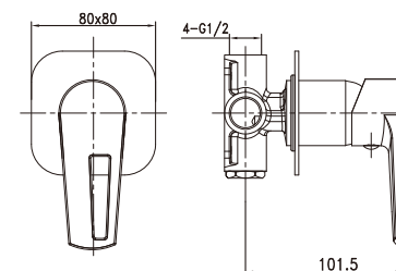
Item Nr. NA1147RB3 Description: Built - in shower mixer. • Brass body. Chrome plating. • \Phi 35mm ceramic cartridge.
