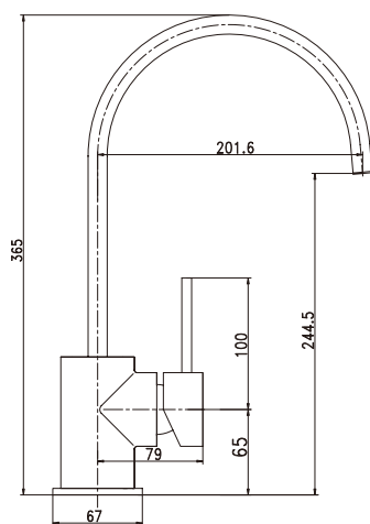
Item Nr. CE045500 Description Kitchen sink mixer • Brass body. Chrome plating. Brass swivel spout. • Ø35mm ceramic cartridge.
