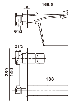
Item Nr. PF1833R0 Description: Wall basin mixer • Brass body.Chrome plating.Brass spout. • Ø35mm ceramic cartridge.
