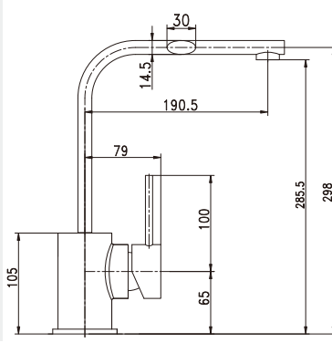
Item Nr. CE045500 Description Kitchen sink mixer • Brass body. Chrome plating. Brass swivel spout. • Ø35mm ceramic cartridge.
