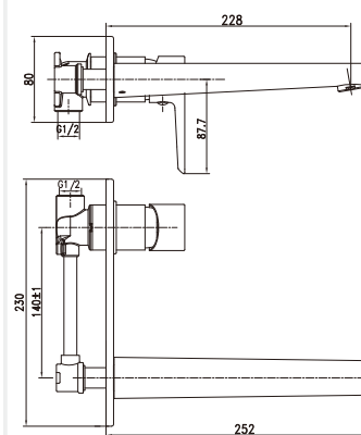
Item Nr. NA1143R3 Description: Wall basin mixer. • Brass body. Chrome plating. Brass spout. • \Phi 35mm ceramic cartridge.
