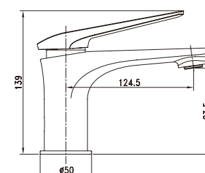
Item Nr.: PF183300 Bronze or Copper finish Description: Basin mixer • Brass body. Bronze or Copper finish. • Ø35mm ceramic cartridge.
